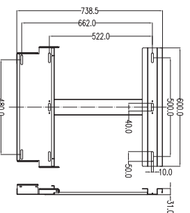
(The dimensions of mounting bracket)
