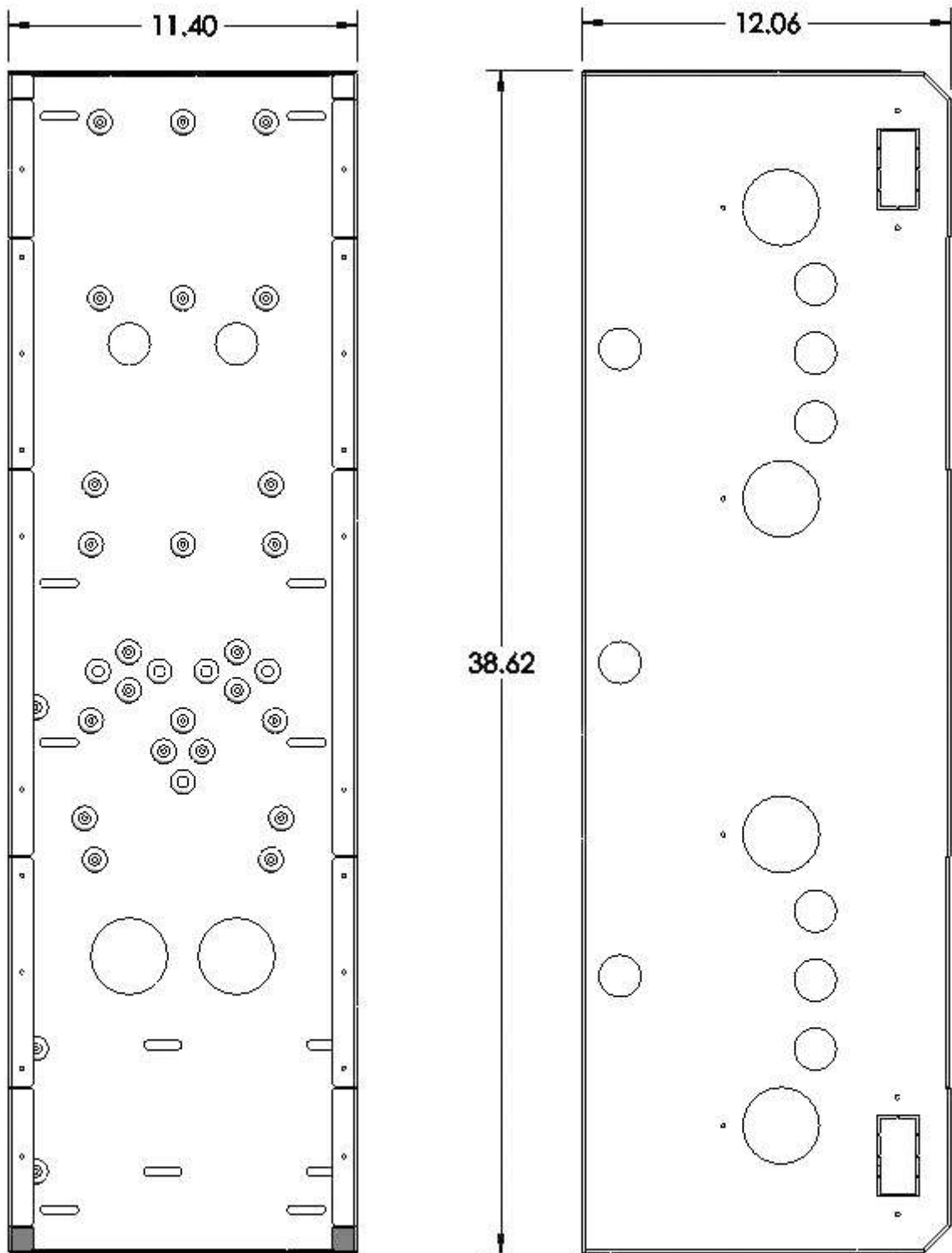
Figure 2: Front View
